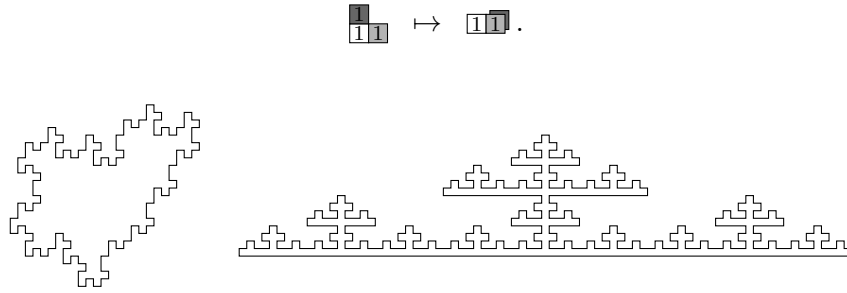
Figure 1: The boundaries of the patterns \sigma^{12}(\{(0,0), 3, [(1,0), 1], [(1,1), 2]\}) of Example 2.3 (left), and \sigma^4(\{(0,0), 1\}) of Example 4.5 (right).
